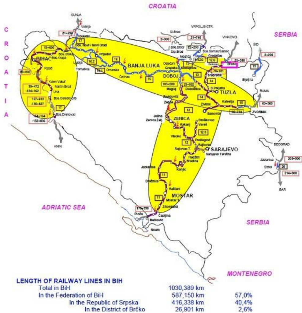
M A P OF RAILWAY SECTIONS TO BE COVERED WITH RECONSTRUCTION OF ELECTRO-ENERGETIC FACILITIES
